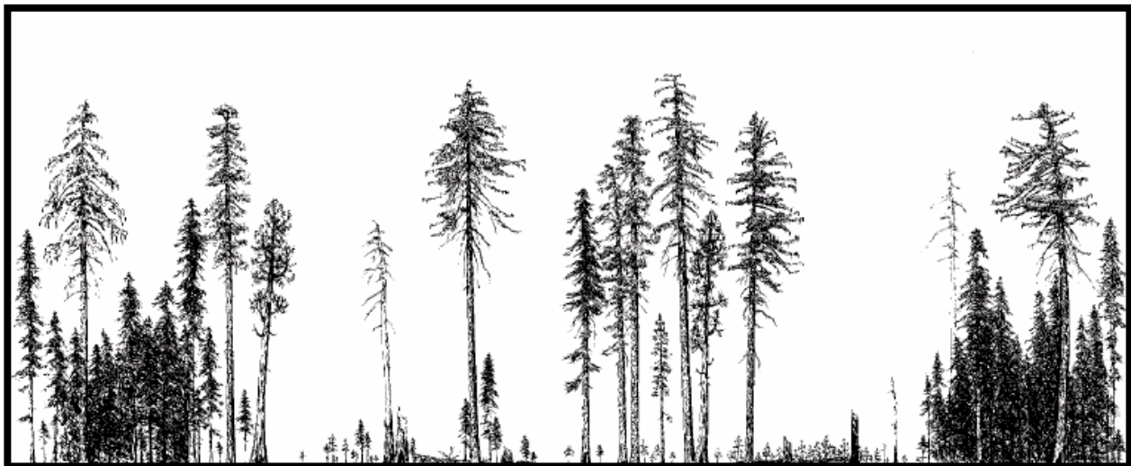
Figure 1. Schematic cross section of a typical pre-settlement mixed conifer forest in the Western Sierra Nevada. From the Sierra Nevada Ecosystem Project (SNEP 1996, drawing by Robert Van Pelt).
